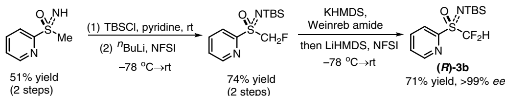
Figure 2 | Synthesis of ( R )- 3b . HMDS, hexamethyldisilazide; TBS, tert-butyldimethylsilyl; NFSI, N-fluorobenzenesulfonimide.
