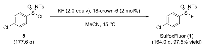
Scheme 6. Hectogram Scale Synthesis of SulfoxFluor (1) from Compound 5
