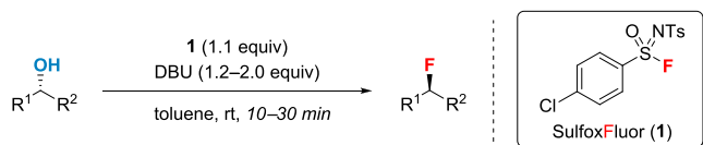
Scheme 1. Deoxyfluorination of Alcohols with SulfoxFluor ( 1 )
