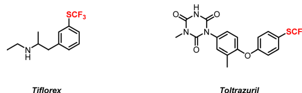
Fig. 1 Examples of SCF 3 -containing drugs.
