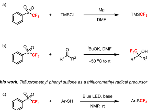
Scheme 1 Trifluoromethylations with trifluoromethyl phenyl sulfone.
