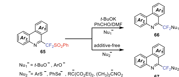
Scheme 17. Radical (phenylsulfonyl)difluoromethylation of isocyanides and their transformations.
