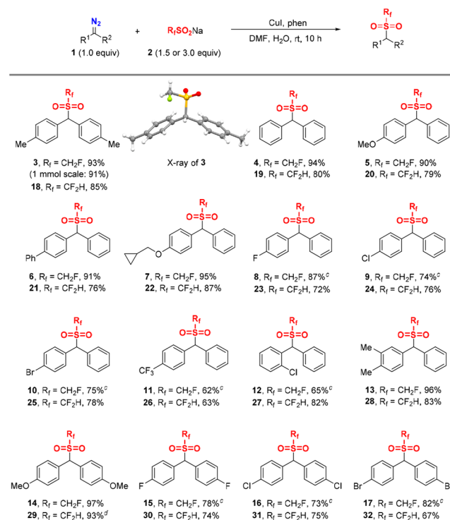
Scheme 2. Scope of Diazo Compounds a,b
