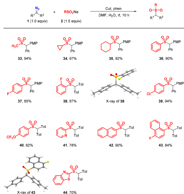
Scheme 3. Scope of Sulfinate Salts a,b
