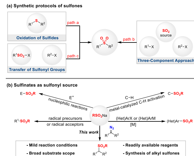
Scheme 1. Strategies for the Synthesis of Sulfones
