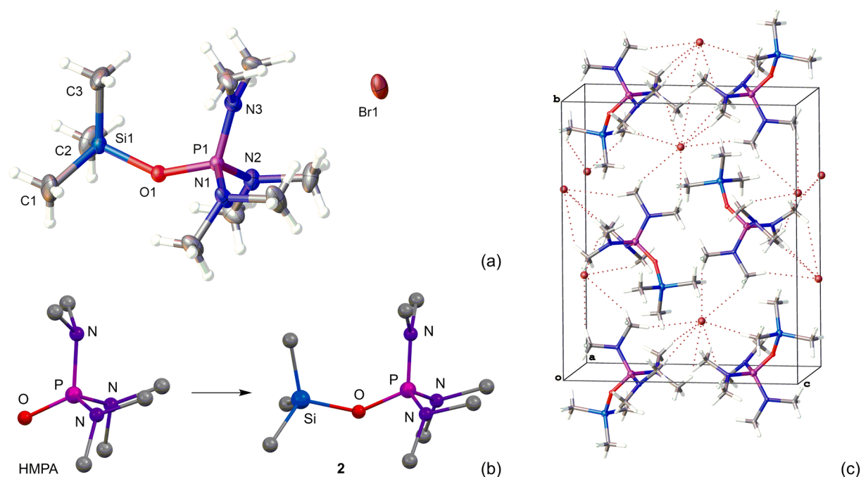
Fig. 2. (a) Molecular structure of salt 2. Atoms are presented as ellipsoids of anisotropic displacement (50% probability). (b) Comparison of crystal structures of HMPA and salt 2, hydrogen atoms are mitted. (c) Crystal packing of salt 2. Selected parameters (Å, deg.): P1-O1 1.5448(16), P1-N3 1.602(2), P1-N2 1.620(2), P1-N1 1.621(2), Si1-O1 1.6865(17), Si1-C1 1.844(3), P1-O1-Si1-144.19(11), O1-P1-N3 117.35(10), O1-P1-N2 104.42(10). Unit cell monoclinic, space group P2_1/c , a = 8.4505(14) , b = 15.185(3) , c = 12.913(2) , \beta = 92.776(4) .
