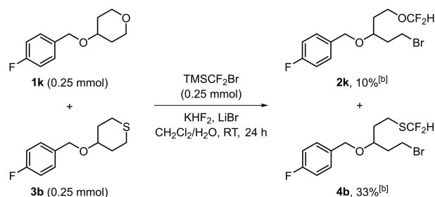
Scheme 5. Mechanistic investigations. [a] The yields were determined by 1 H NMR analysis using PhOCF 3 as an internal standard (for details, see the Supporting Information). [b] The yields were determined by 19 F NMR analysis using PhOCF 3 as an internal standard.
