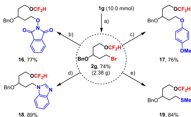
Scheme 4. Scale-up synthesis and synthetic application of bromination product 2g . Conditions: a) TMSCF 2 Br (3.0 equiv.), KHF 2 /LiBr, CH 2 Cl 2 /H 2 O, RT; b) 1 H -benzo[d]imidazole, NaH, THF, 60 °C; c) 4-MeOC 6 H 4 OH, NaH, DMF, RT; d) 2-hydroxyisindoline-1,3-dione, DBU, 80 °C; e) MeSNa, THF, 60 °C.
