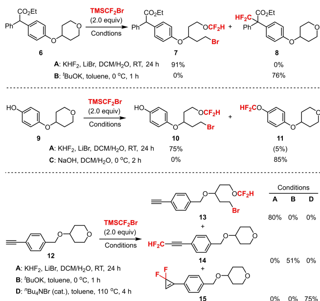
Scheme 3. Orthogonal transformations of ambident cyclic ether-containing substrates. The yields refer to isolated yields of analytically pure products. The yield in the parentheses refers to 19 F NMR yield of the side product that was confirmed by GC-MS analysis.
