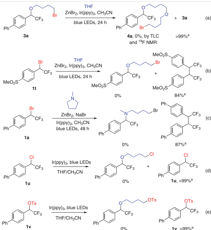
Scheme 3 Additional experiments. a Yield determined by ^{19}\text{F} NMR spectroscopy.
