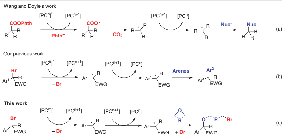
Scheme 1 Two redox-neutral patterns to form carbocation under photoredox catalysis conditions
