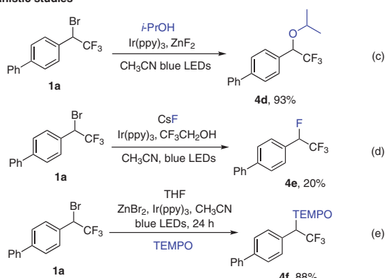
Scheme 4 Applications of product 3q and mechanistic studies.
