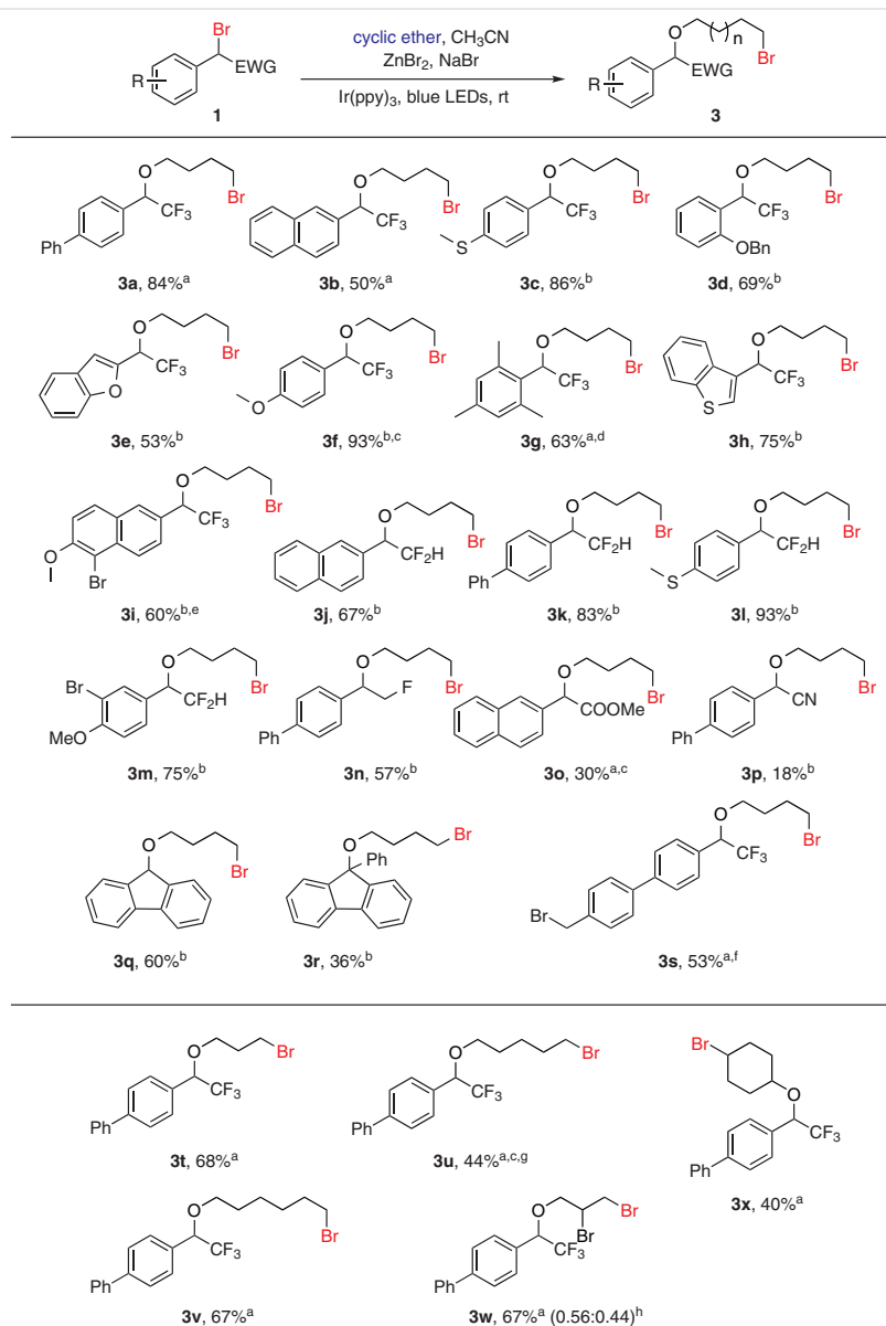
Scheme 2 Scope of the substrates. a Unless otherwise mentioned, the reaction conditions are as follows: 1 (0.5 mmol), ZnBr 2 (0.5 equiv), NaBr (0.45 equiv), cyclic ethers (5 equiv), Ir(ppy) 3 (0.5 mol%) in CH 3 CN (5 mL) for 24 h. b 1 (0.5 mmol), Ir(ppy) 3 (1 mol%), CH 3 CN (2.5 mL)/THF (2.5 mL) for 48 h. c 7 days. d 0.4 equiv of NaBr, 3 days. e 0.4 mmol scale. f NaBr (0.4 equiv), THF (10 equiv), Ir(ppy) 3 (1 mol%) in CH 3 CN (5 mL) for 48 h. g 1 mol% Ir(ppy) 3 . h Ratio of diastereoisomers, determined by 19 F NMR spectroscopy.
