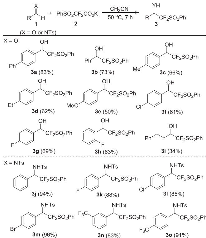
Scheme 2. (Phenylsulfonyl)difluoromethylation of aldehydes and imines. Reaction conditions: substrate 1 (0.5 mmol) and 2 (0.75 mmol) in \text{CH}_3\text{CN} (5 mL) at 50^\circ\text{C} for 7 h. All yields were isolated yields.
