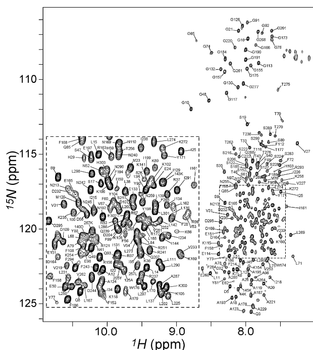
Figure 1. Backbone amide resonance assignments of GGC. The two-dimensional [ 15 N- 1 H] TROSY-HSQC spectrum of U- 2 H, 15 N, 13 C]-GGC in DPC micelles shown here was collected on a Bruker 600 MHz spectrometer with a cryogenic probe at 30 °C. Sequence-specific resonance assignments are indicated by the residue labels. To resolve the peaks in the crowded region, the spectrum was over-processed with a sharp apodization function in the 1 H dimension with a 63°-shifted squared sine-bell window.
