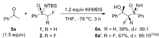
Scheme 3. Different reactivities of 1 and 2 towards 5a .
