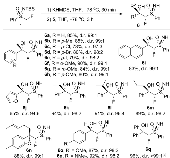
Scheme 4. Stereoselective monofluoromethylation of ketones and aldehydes with sulfoximine 1 . General procedures: under N 2 , KHMDS (1 M in THF, 2.5 mL, 2.5 mmol) was added to the solution of 1 (287 mg, 1 mmol) in THF (5 mL) at -78^{\circ}\text{C} ; 30 min later, a solution of 5 (2 mmol) in THF (1 mL) was added, and 3 hours later, the reaction was quenched with 5 mL of 3 M HCl (aq). The d.r. value was determined by 19 F NMR spectroscopy before silica gel column chromatography and refers to the facial selectivity unless otherwise noted. Yield refers to the yield of the isolated major diastereoisomer. [a] The d.r. value results from the sulfur and fluorinated carbon stereogenic centers.
